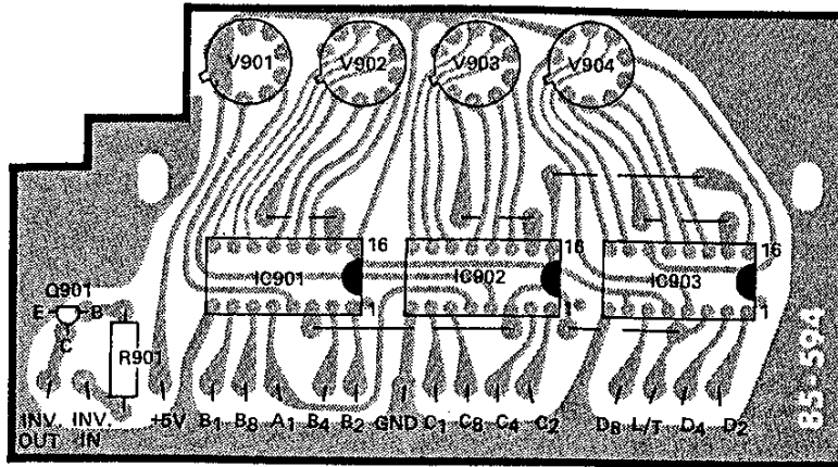
READOUT CIRCUIT BOARD (Viewed from foil side)
