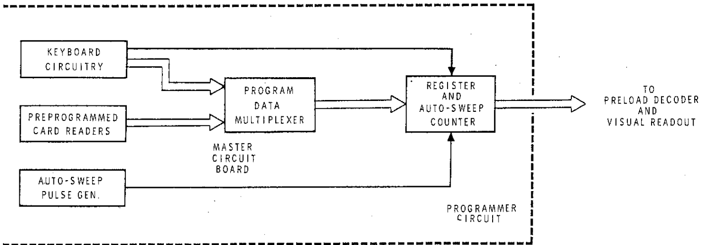
BLOCK DIAGRAM
