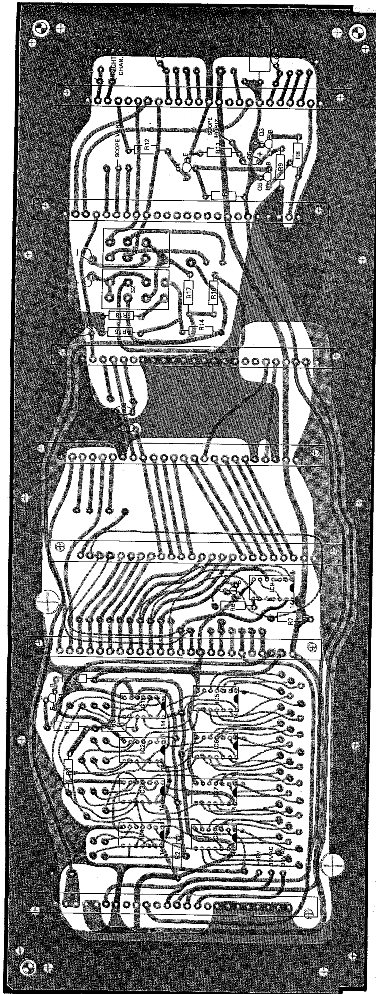
MASTER CIRCUIT BOARD (Viewed from component side)
