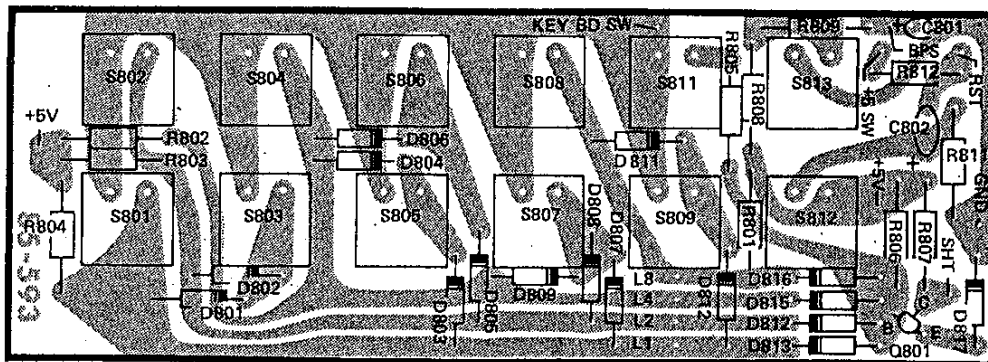
KEYBOARD CIRCUIT BOARD (Viewed from component side)
